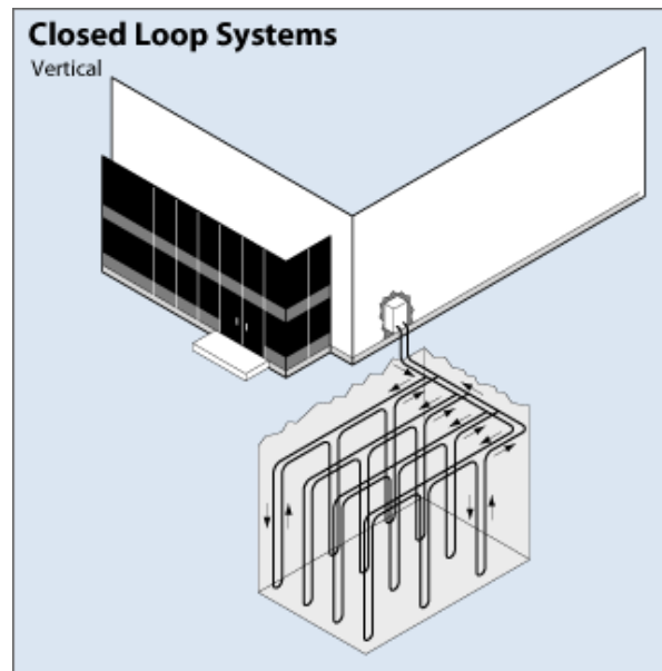
Figure 12. a (above) & b (below) Vertical closed-loop “Ground Source” system for larger structures.
