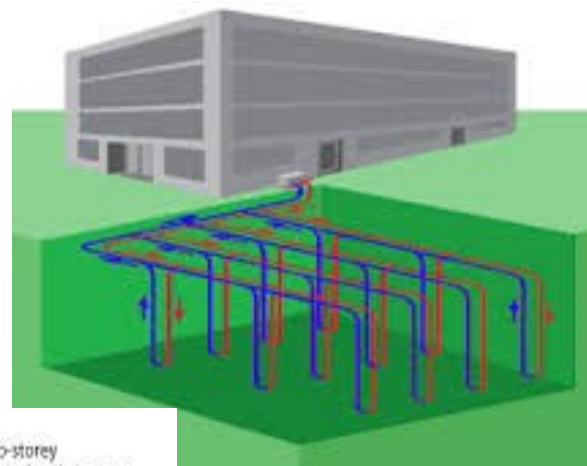
Figure 12. a (above) & b (below) Vertical closed-loop “Ground Source” system for larger structures.
