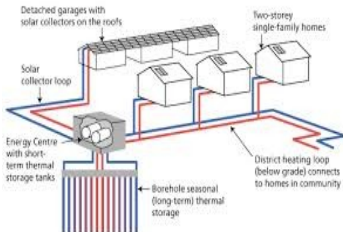
Figure 12. c (below) Vertical closed-loop “Ground Source” system for a small district heating/cooling system.
